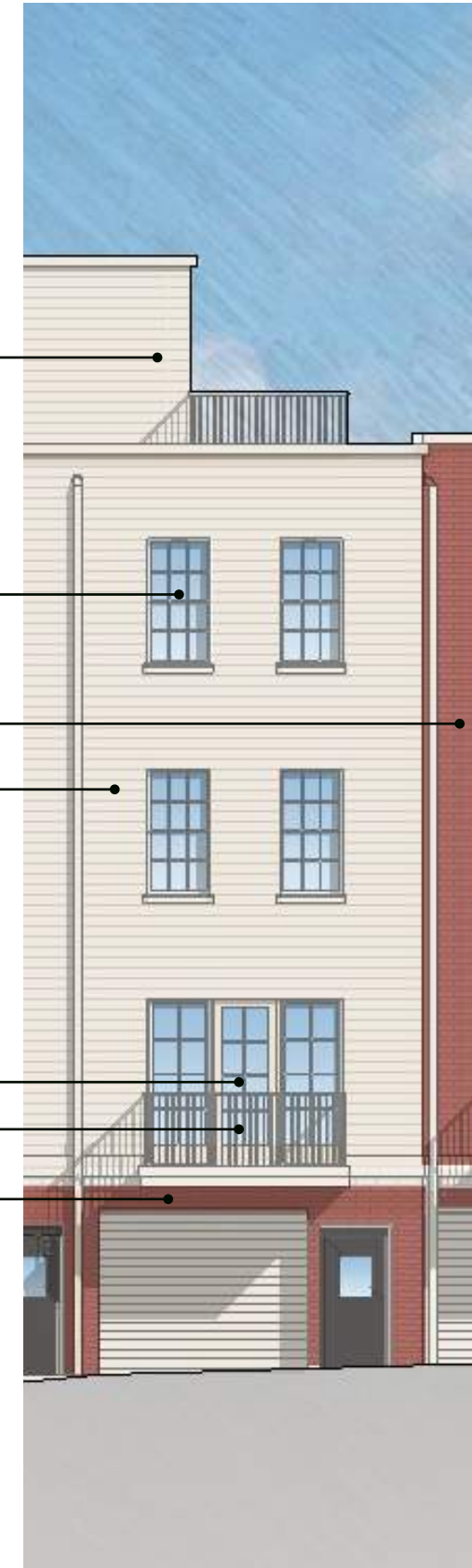
West Elevation
